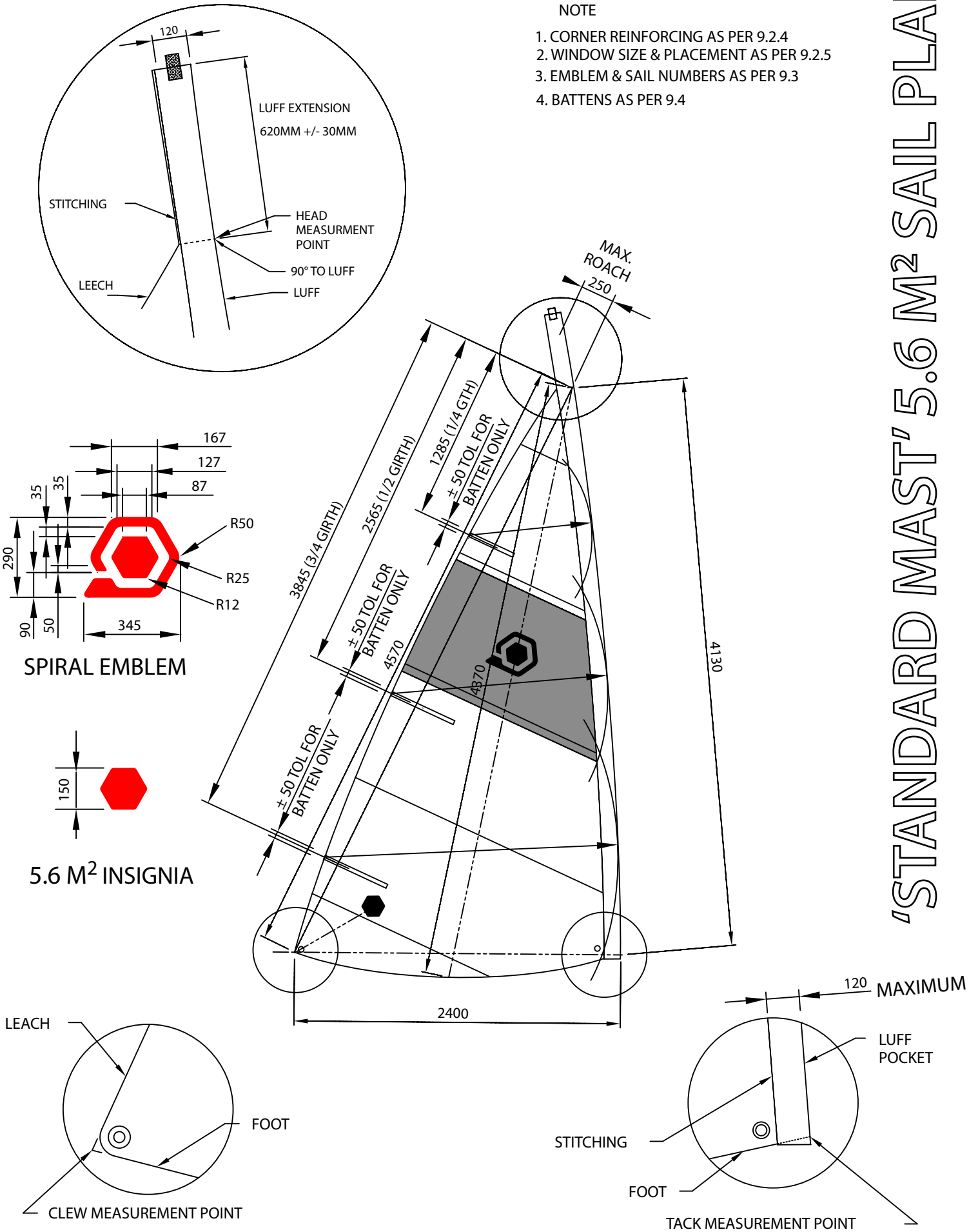
"STANDARD MAST" 5.6 M 2 SAIL PLAN
