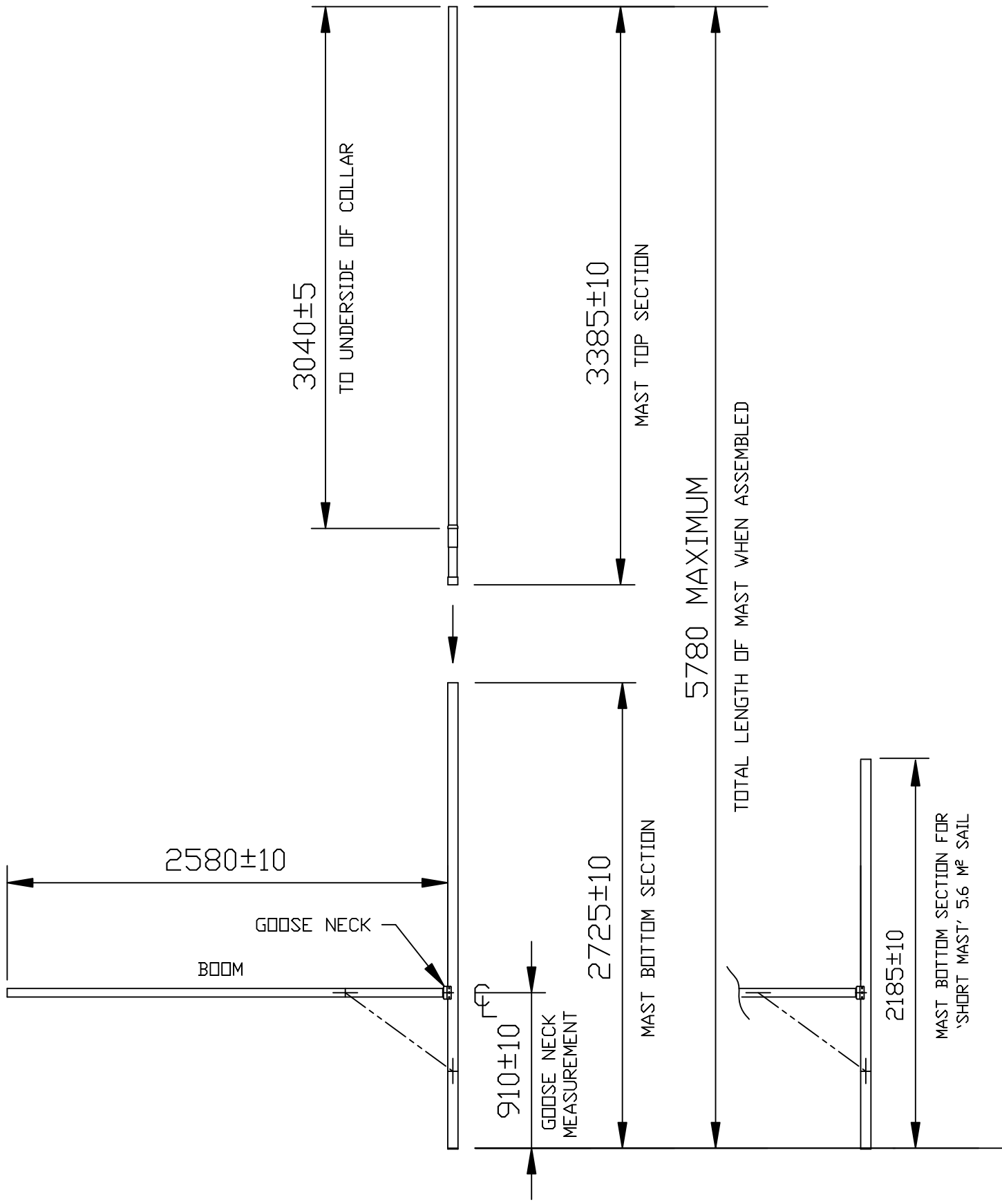
SPAR MEASUREMENT DETAILS (TO BE READ IN CONJUNCTION WITH RULES 10 & 11) FIG. 5
