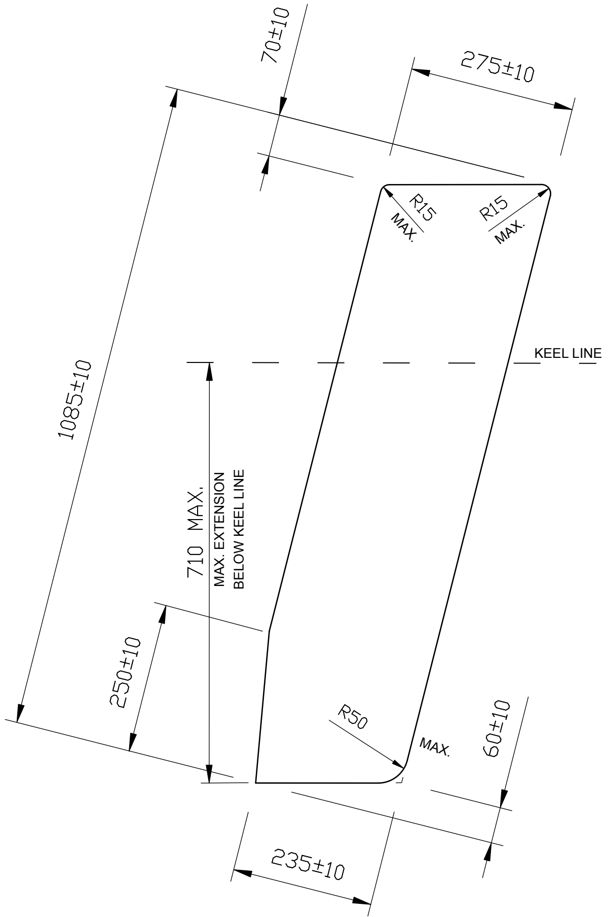
SPIRAL CENTREBOARD MEASUREMENT DETAILS FIG. 4
